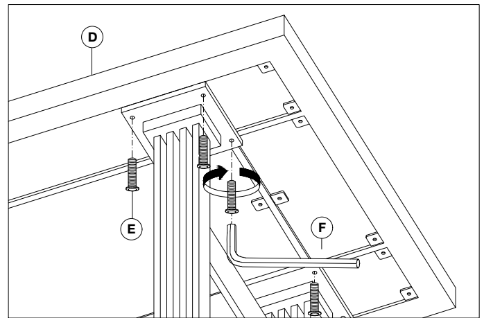
4. Assemble the table top to the stand using bolts (E) and the allen key.
