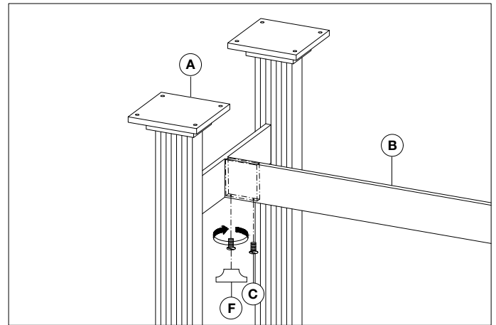
2. Secure the crossbar to the legs with the screws (C).
