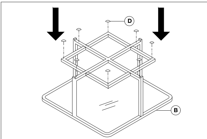
3. Place the rubber cushions.
